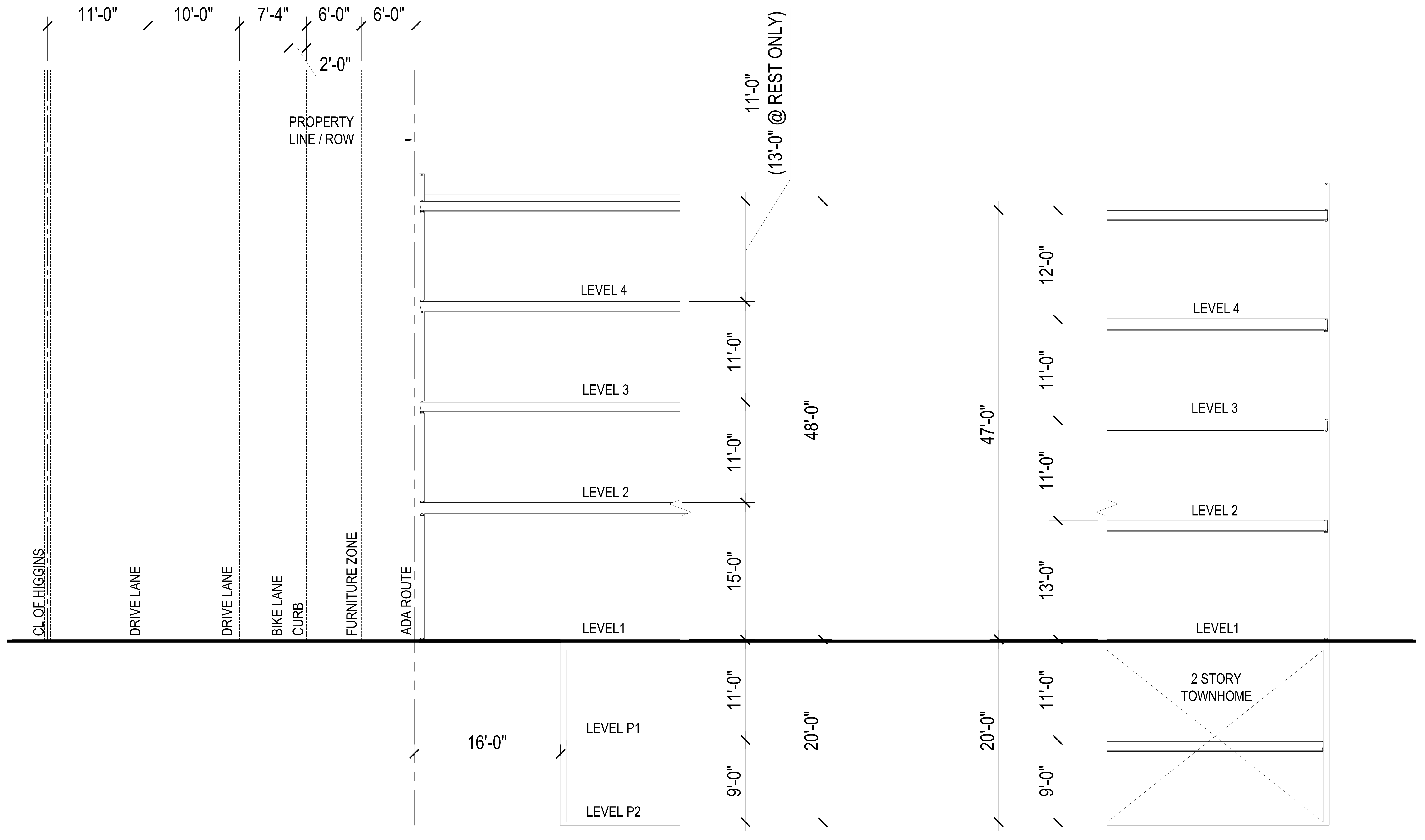
TYPICAL HOTEL SECTION
